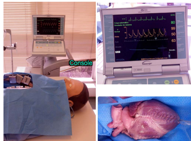
Fig. 9 - The console of intra-aortic balloon pump (Datascope) with the monitor connected to the simulated pulses and positioned aside the dummy.
