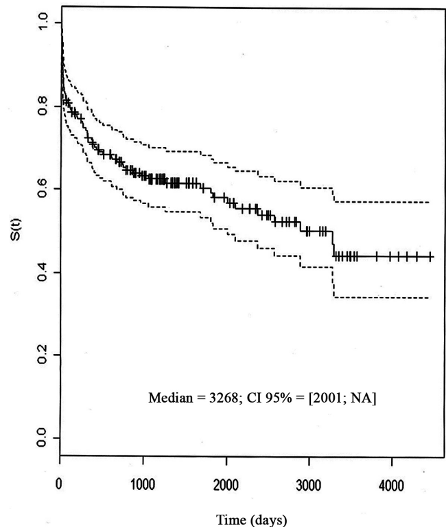
Fig. 1 - Kaplan-Meier curve for the survival time of patients undergoing heart transplant
